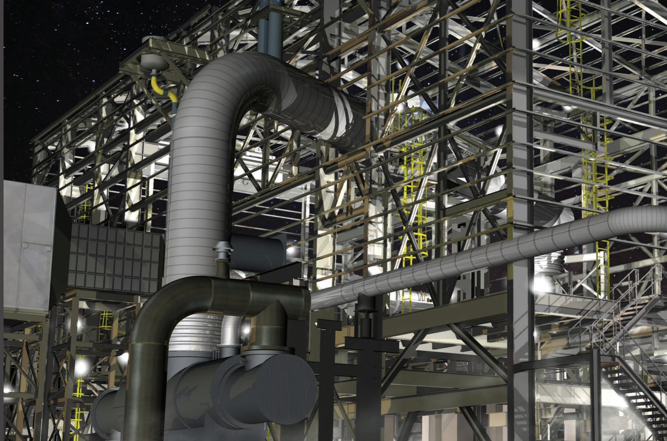
2018 Golden Valve Winner | Photorealism: 3 rd Place | Fandy Maulana Syah Rizal | PT. Rekayasa Industri | Indonesia This rendering represents the under construction structure building for process air compressor and steam turbine for the Banggai Ammonia Plant Project in Indonesia.
