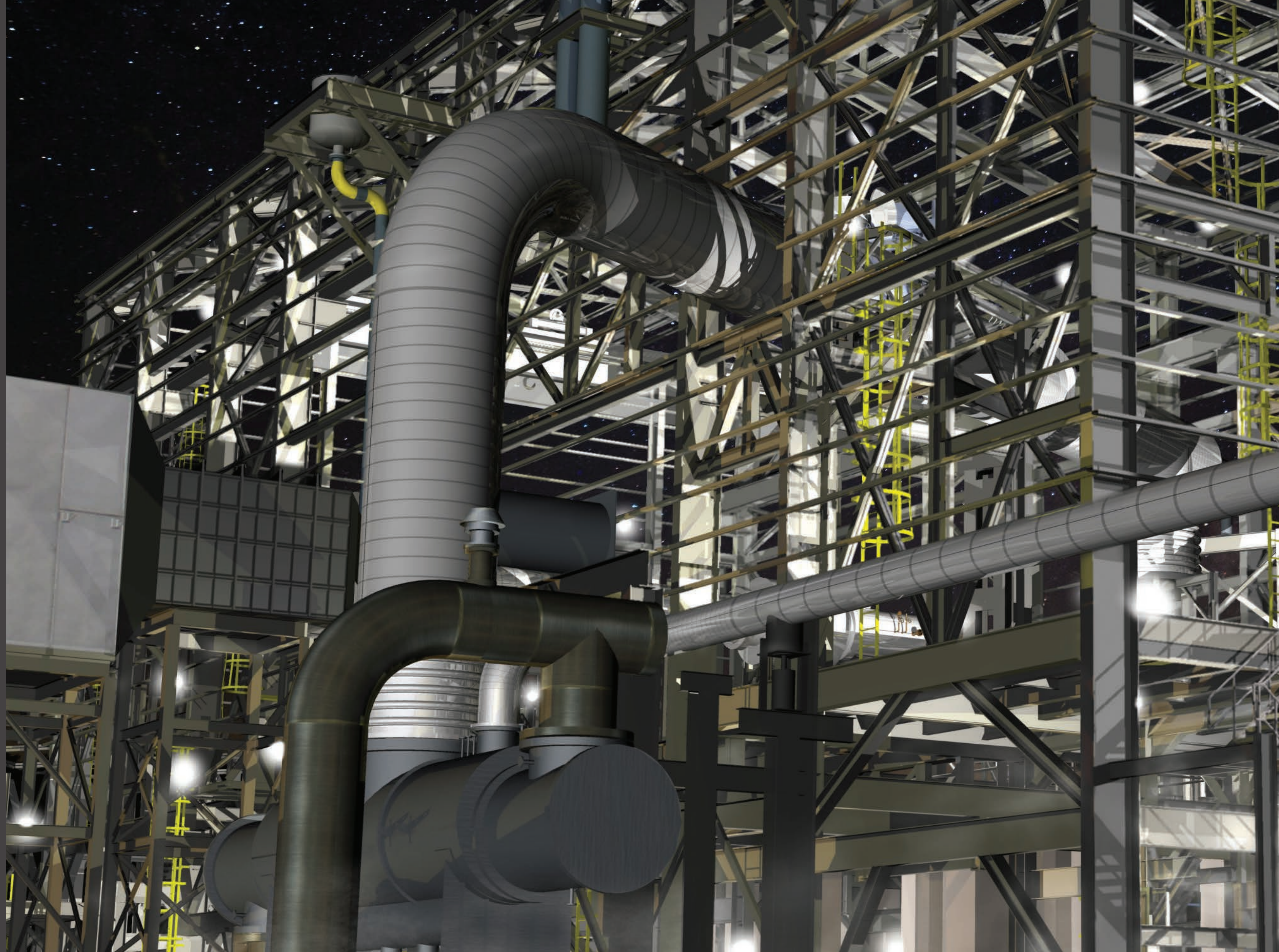
2018 Golden Valve Winner | Photorealism: 3 rd Place | Fandy Maulana Syah Rizal | PT. Rekayasa Industri | Indonesia This rendering represents the under construction structure building for process air compressor and steam turbine for the Banggai Ammonia Plant Project in Indonesia.
